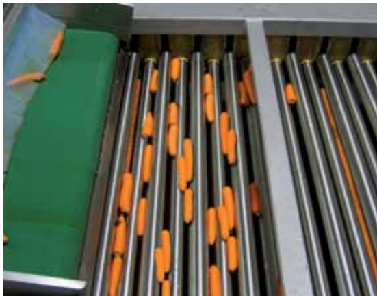
Long produce such as carrots are sized with round polished stainless steel rollers
